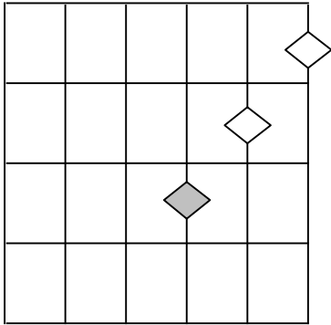
ROOT INVERSION
