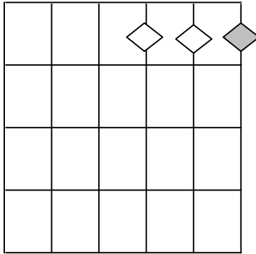
FIRST INVERSION
