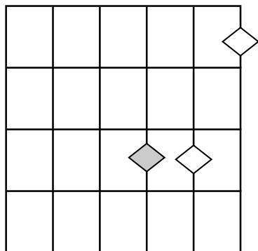
ROOT INVERSION
