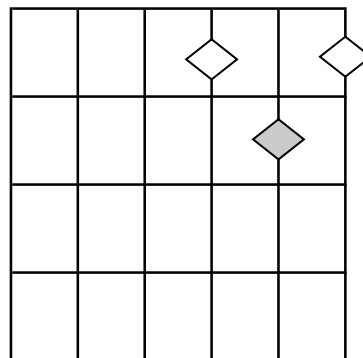
SECOND INVERSION
