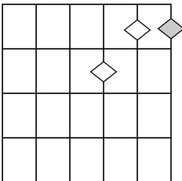
FIRST INVERSION
